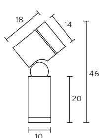
magnetic base
