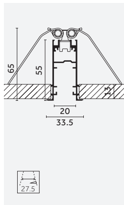
Recessed Trim
