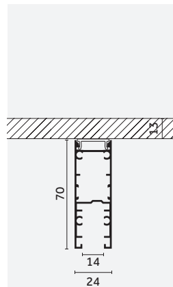
Surface/Pendant
